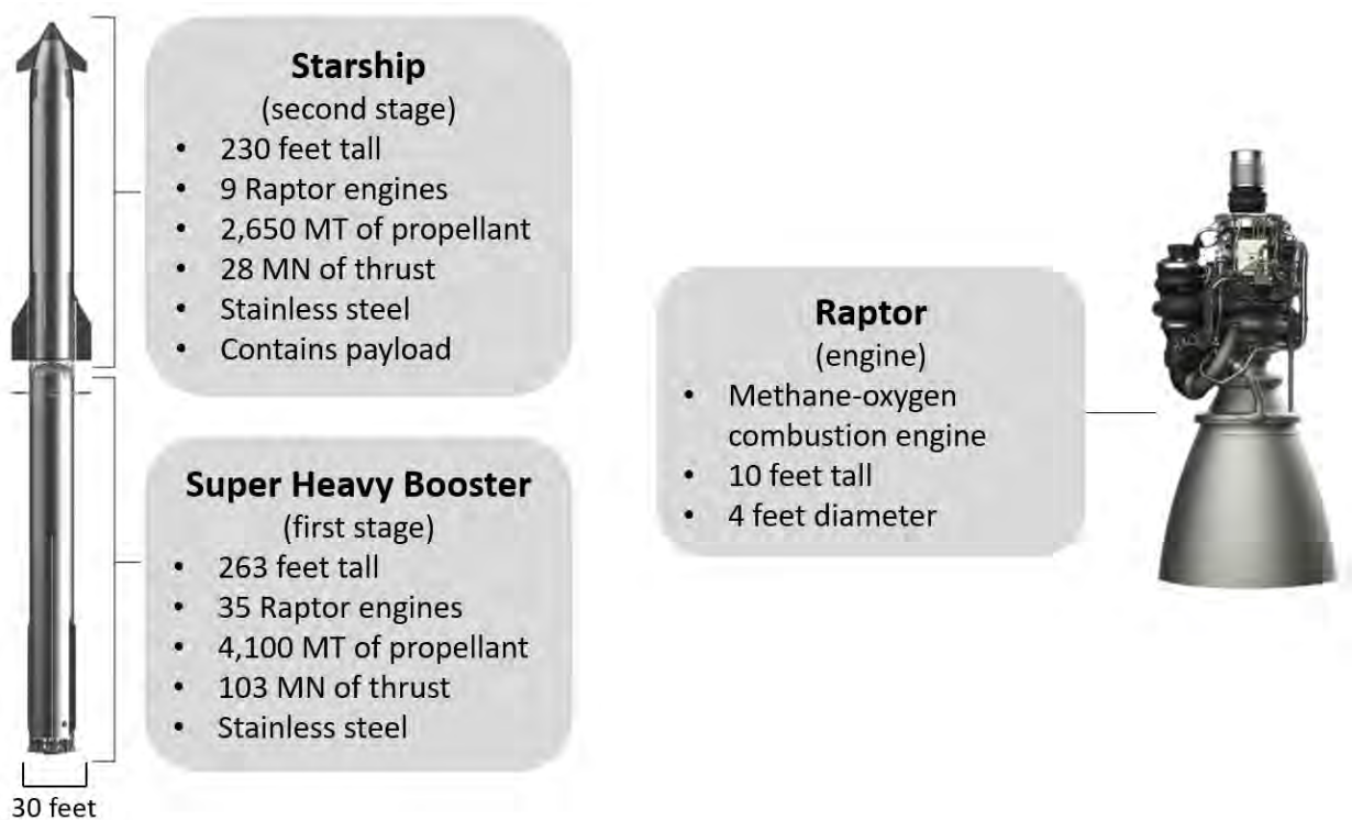
Figure 2-3. Starship-Super Heavy Launch Vehicle Design
